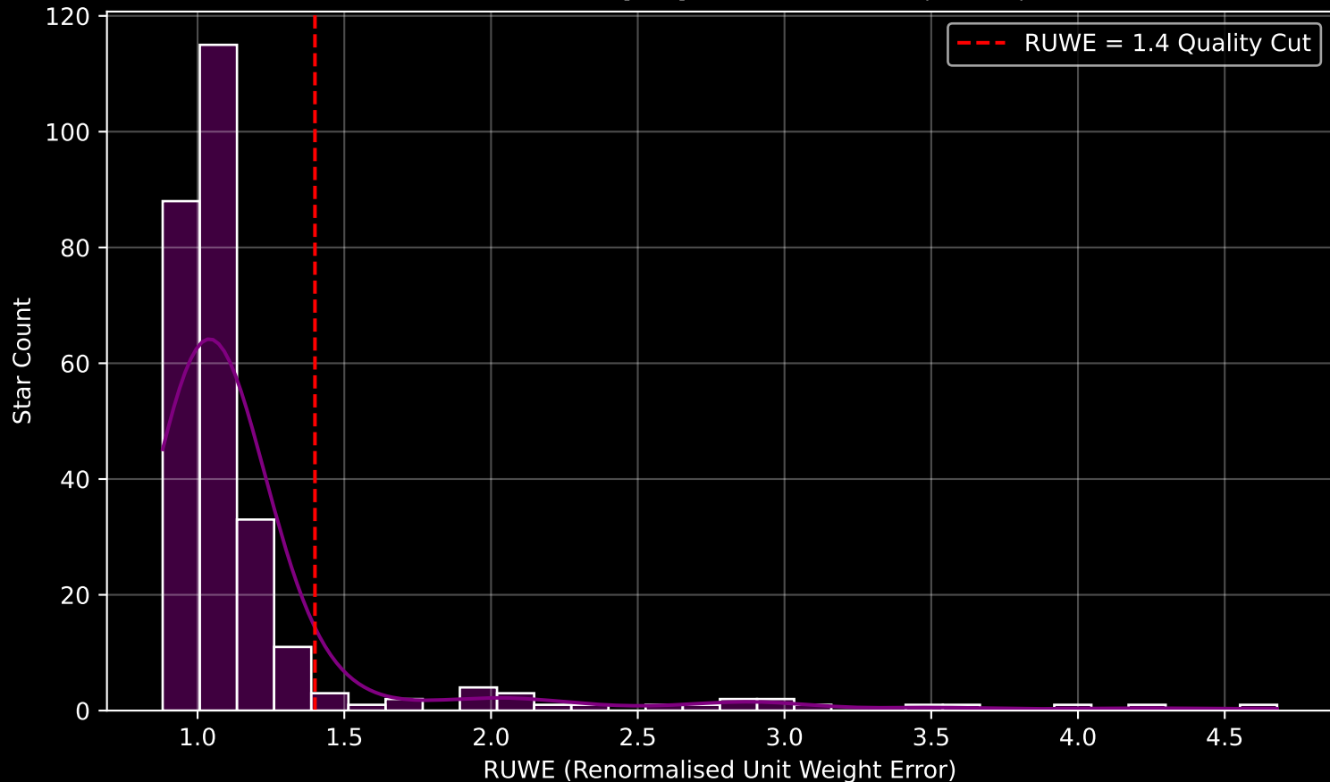
GALAH DR4 Field [358] RUWE Distribution (n= 274)
