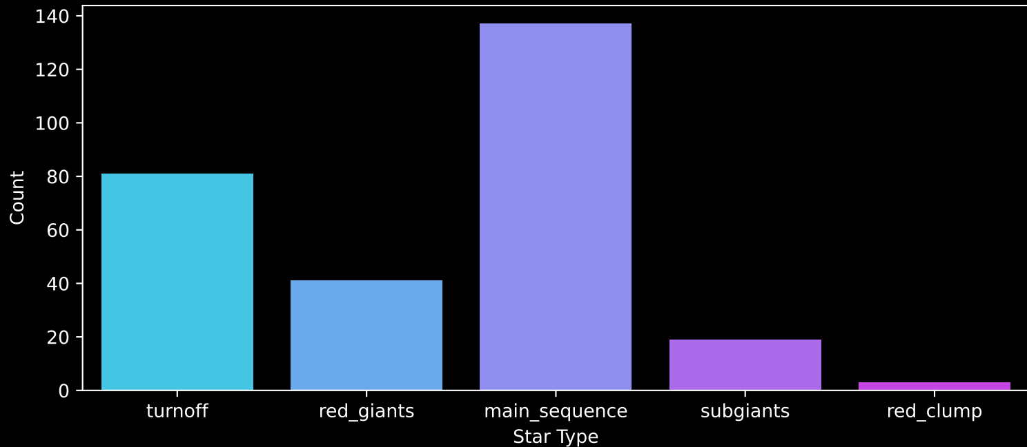
GALAH DR4 Field: [358] Count plot of Star Type
