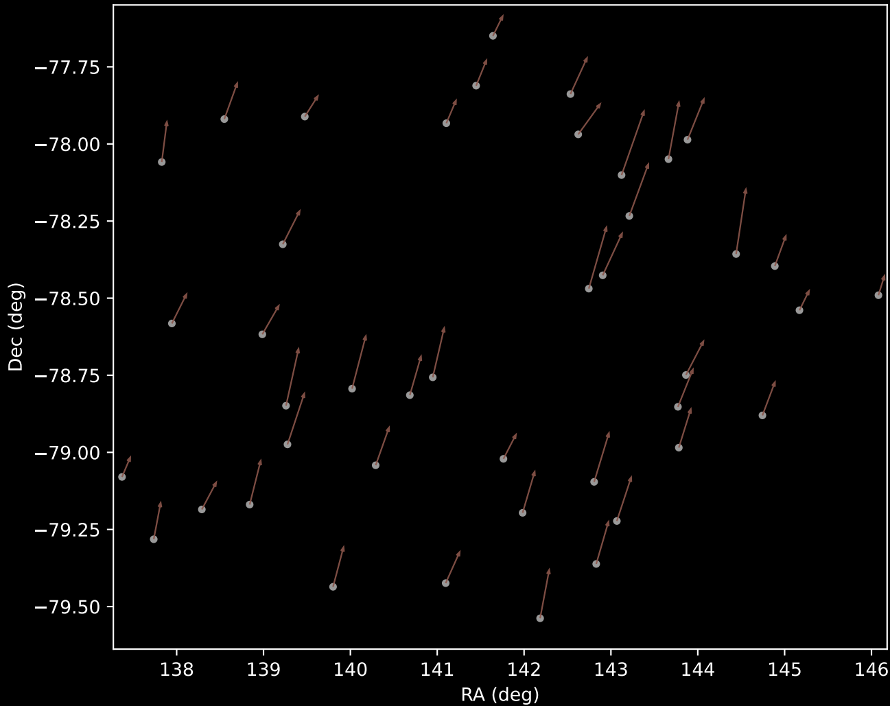
GALAH DR4 Cluster 10 Proper Motion Vectors (n=43)
